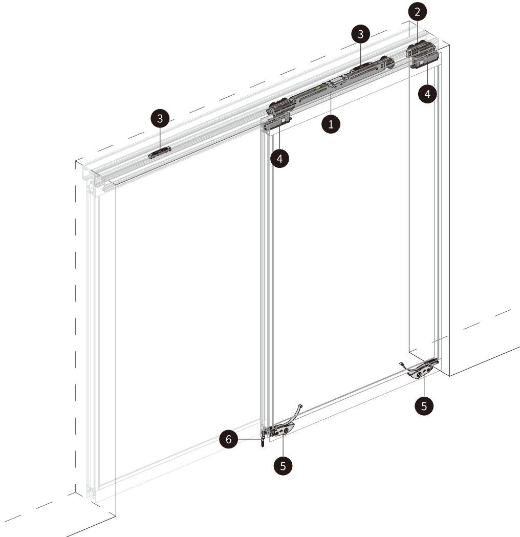
Split sliding roller Installation
