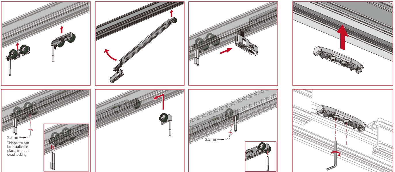
Split sliding roller Installation
